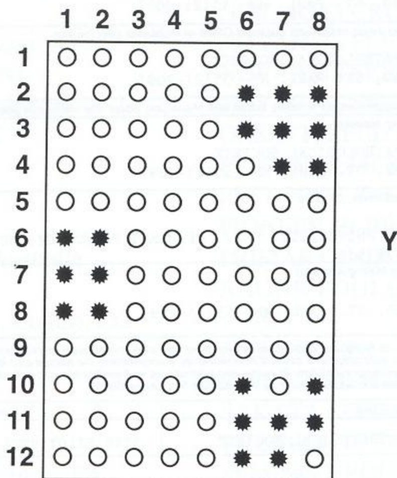
Fig. 2. Hypothetical data set on an 8 \times 12 -rectangular lattice, first introduced by Gray et al. (14). Infected plants are denoted by filled symbols, healthy plants as open circles.
