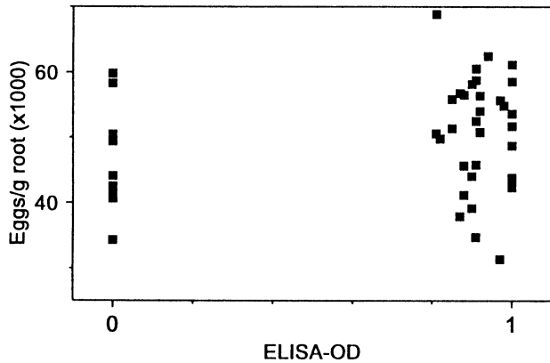
Fig. 4. Reproduction data of Meloidogyne incognita (eggs per gram of root) on tobacco expressing assembled 6D 4 heavy and light chain protein (ELISA-OD around 1) and tobacco expressing either heavy or light chain protein of 6D 4 (ELISA-OD of 0) measured in leaf tissue.
